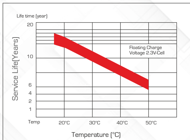
Service (Float) Life and Temperature
